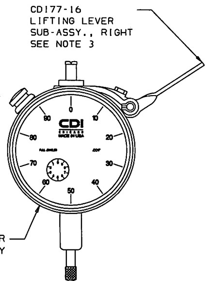
R.H. FRONT VIEW
