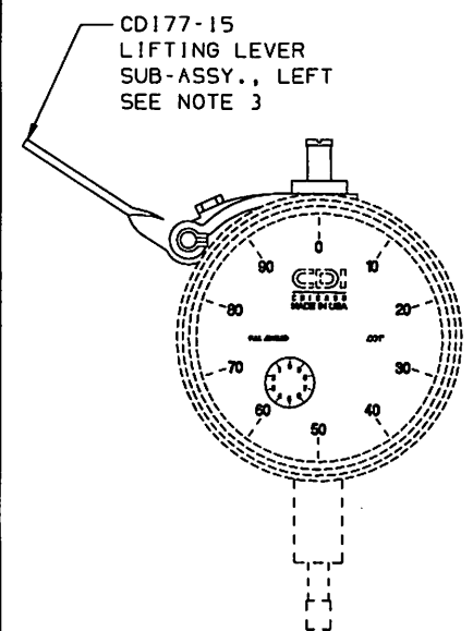
L.H. FRONT VIEW
