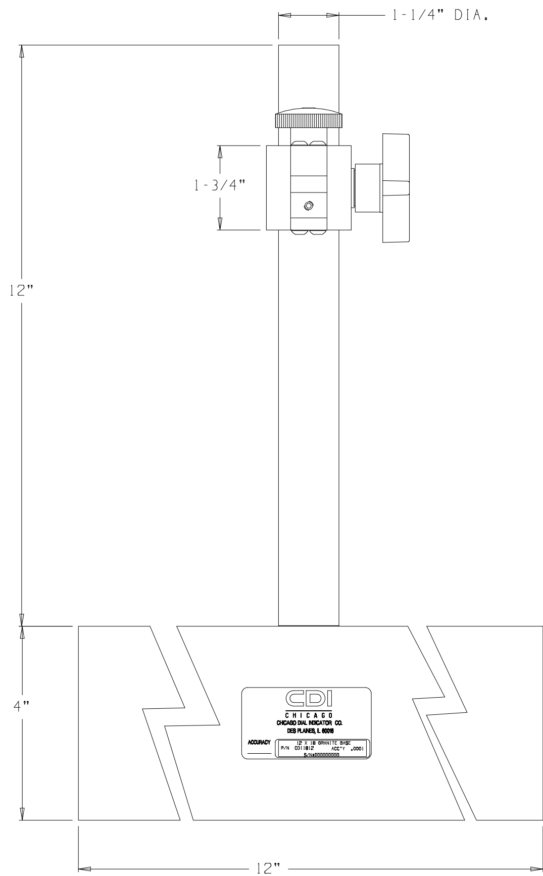
(61812-1S) GRANITE BASE 12" X 18" X 4" W/ADJUSTABLE ARM, STEM MOUNT
