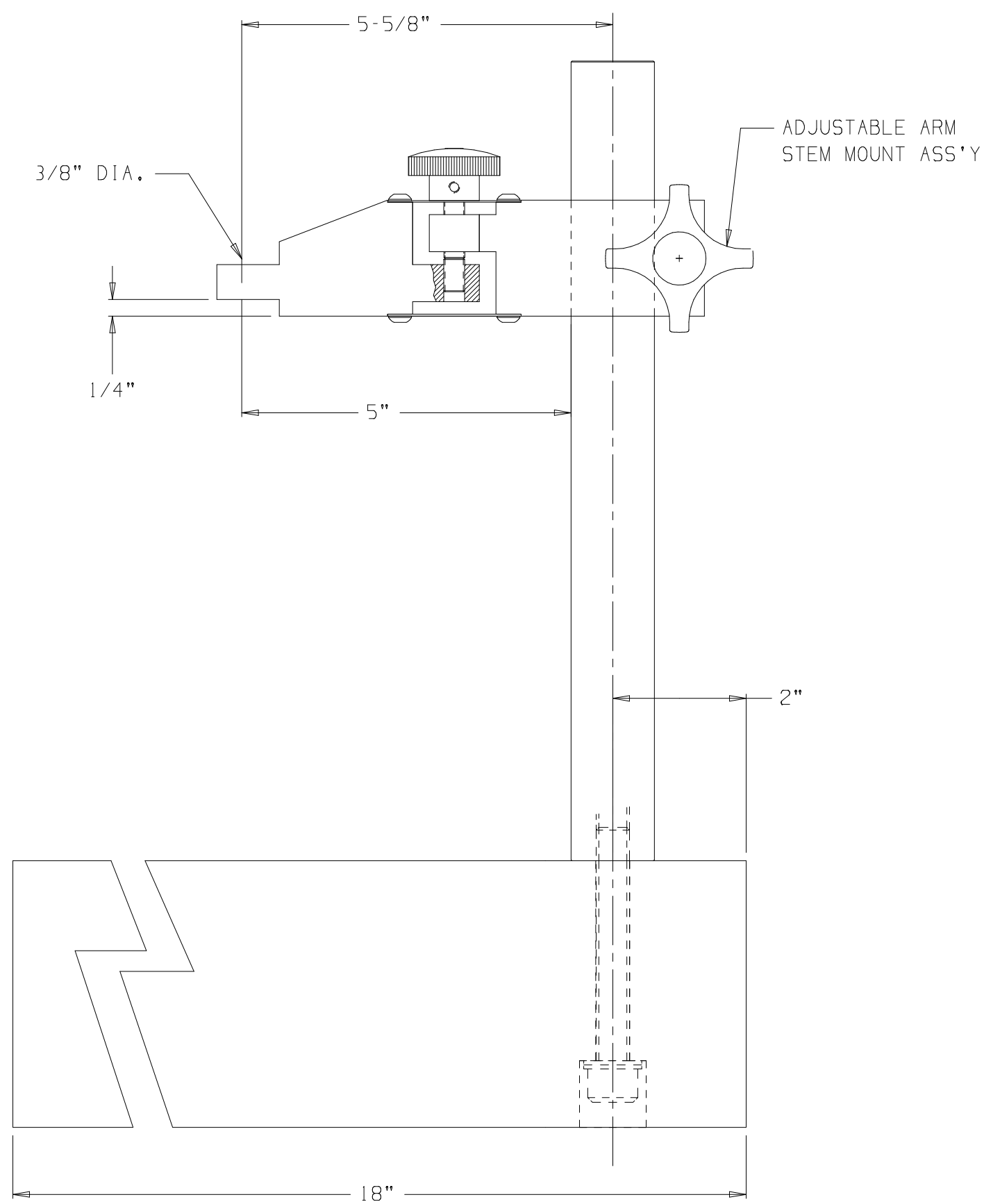
(61812-1S) GRANITE BASE 12" X 18" X 4" W/ADJUSTABLE ARM, STEM MOUNT
