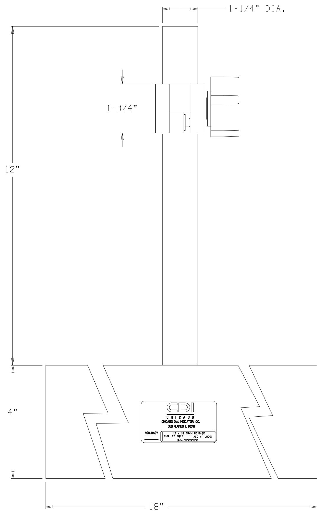
(61812-1R) GRANITE BASE 18" X 12" X 4" W/RIGID ARM, LUG MOUNT
