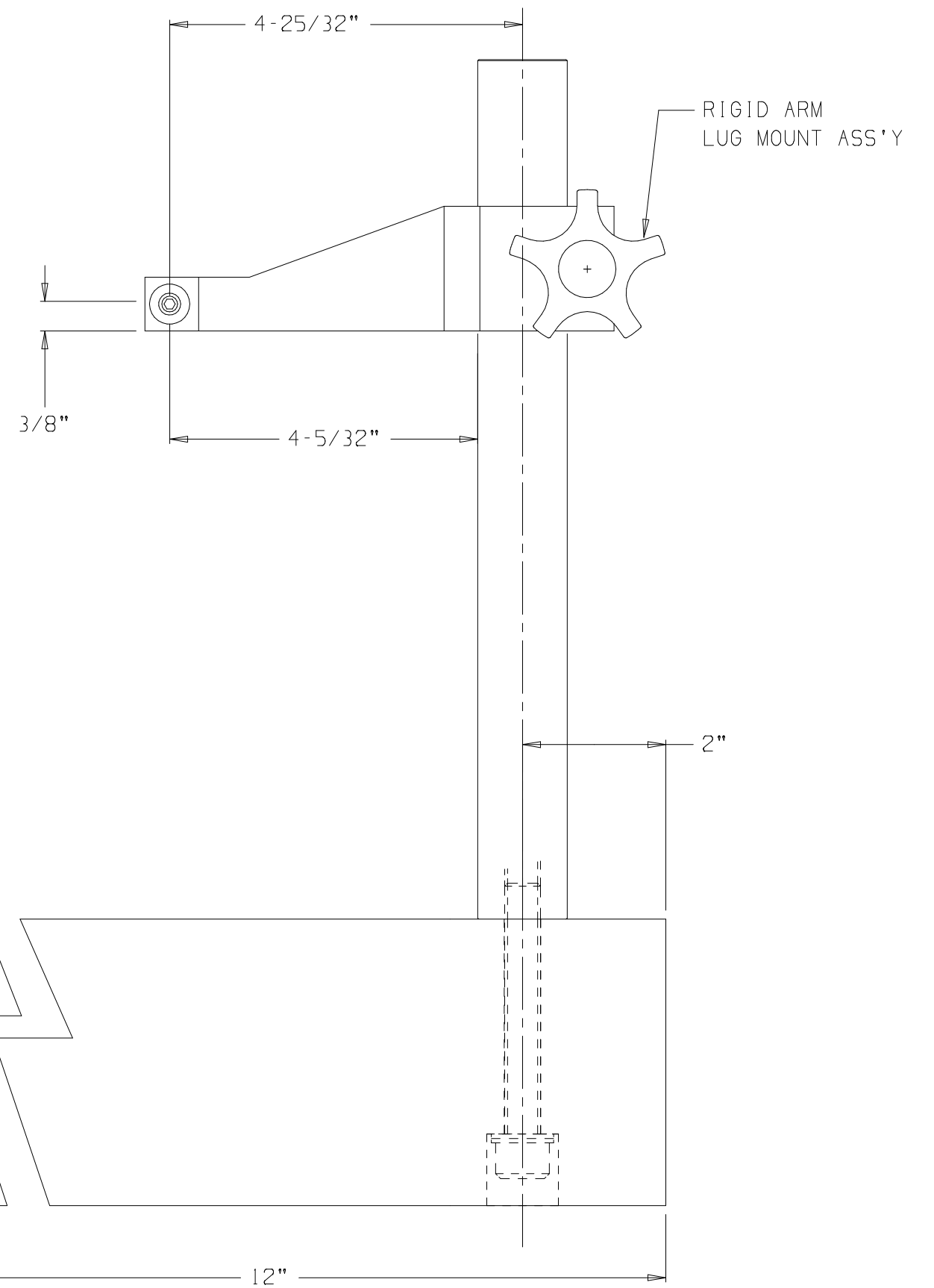
(61812-1R) GRANITE BASE 18" X 12" X 4" W/RIGID ARM, LUG MOUNT
