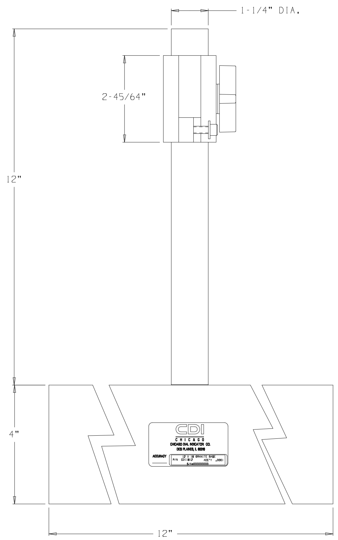
(61812-1R) GRANITE BASE 12" X 18" X 4" W/RIGID ARM, LUG MOUNT
