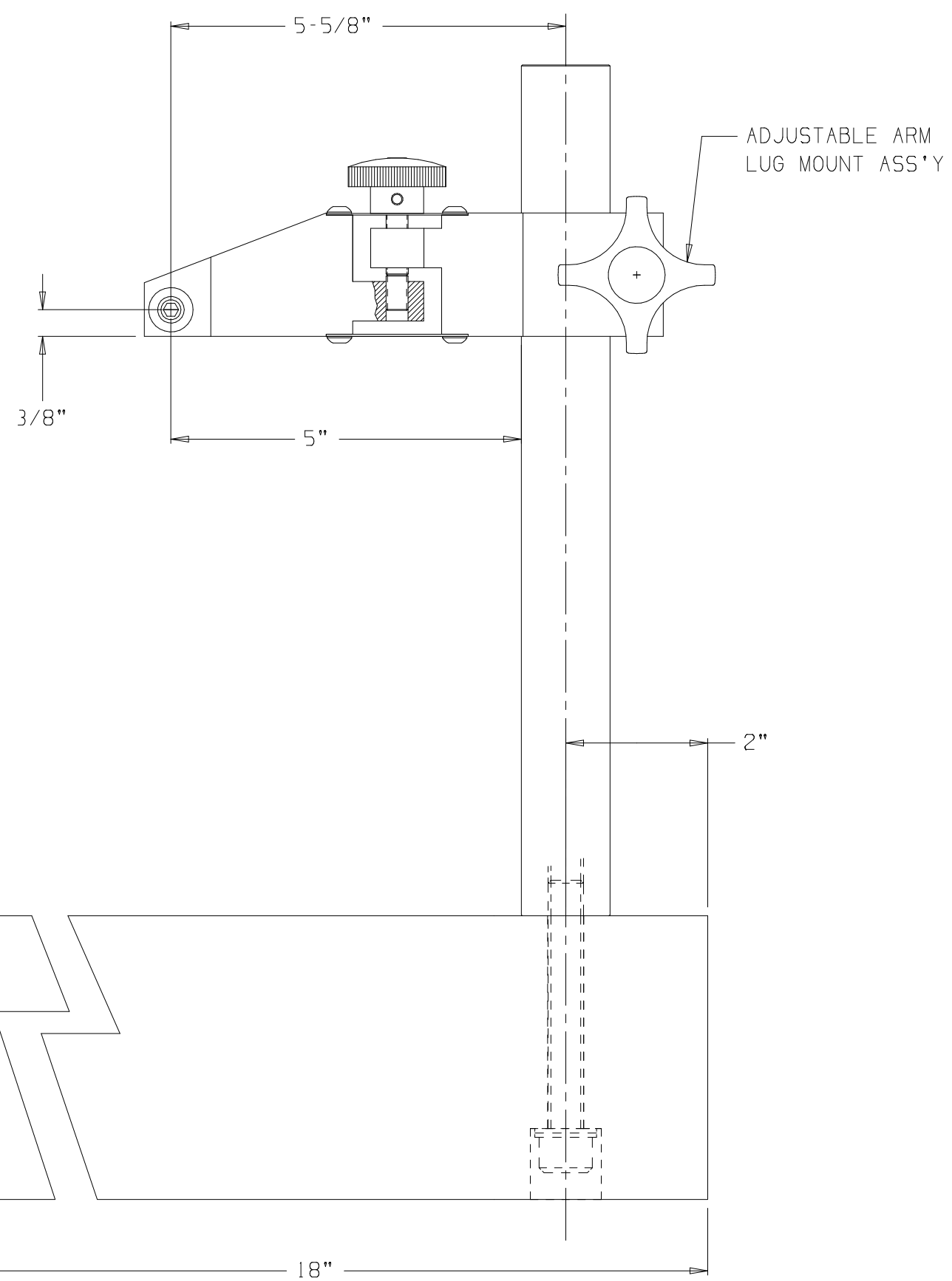
(61812-1) GRANITE BASE 12" X 18" X 4" W/ADJUSTABLE ARM, LUG MOUNT
