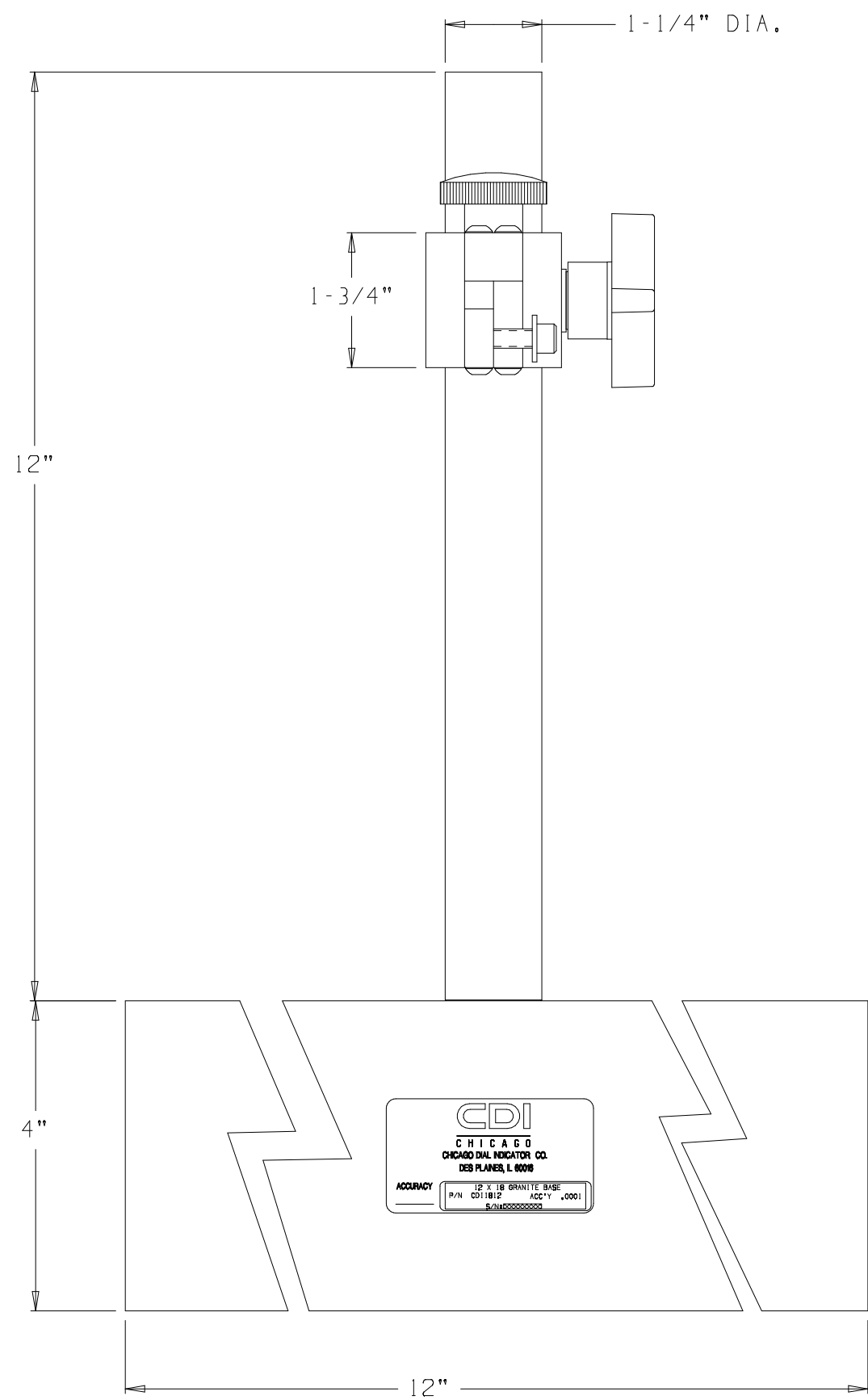
(61812-1) GRANITE BASE 12" X 18" X 4" W/ADJUSTABLE ARM, LUG MOUNT
