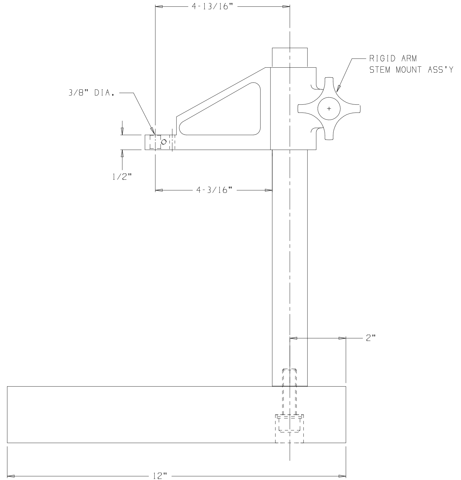
(60812-1RS) GRANITE BASE 8" X 12" X 2" W/RIGID ARM, STEM MOUNT
