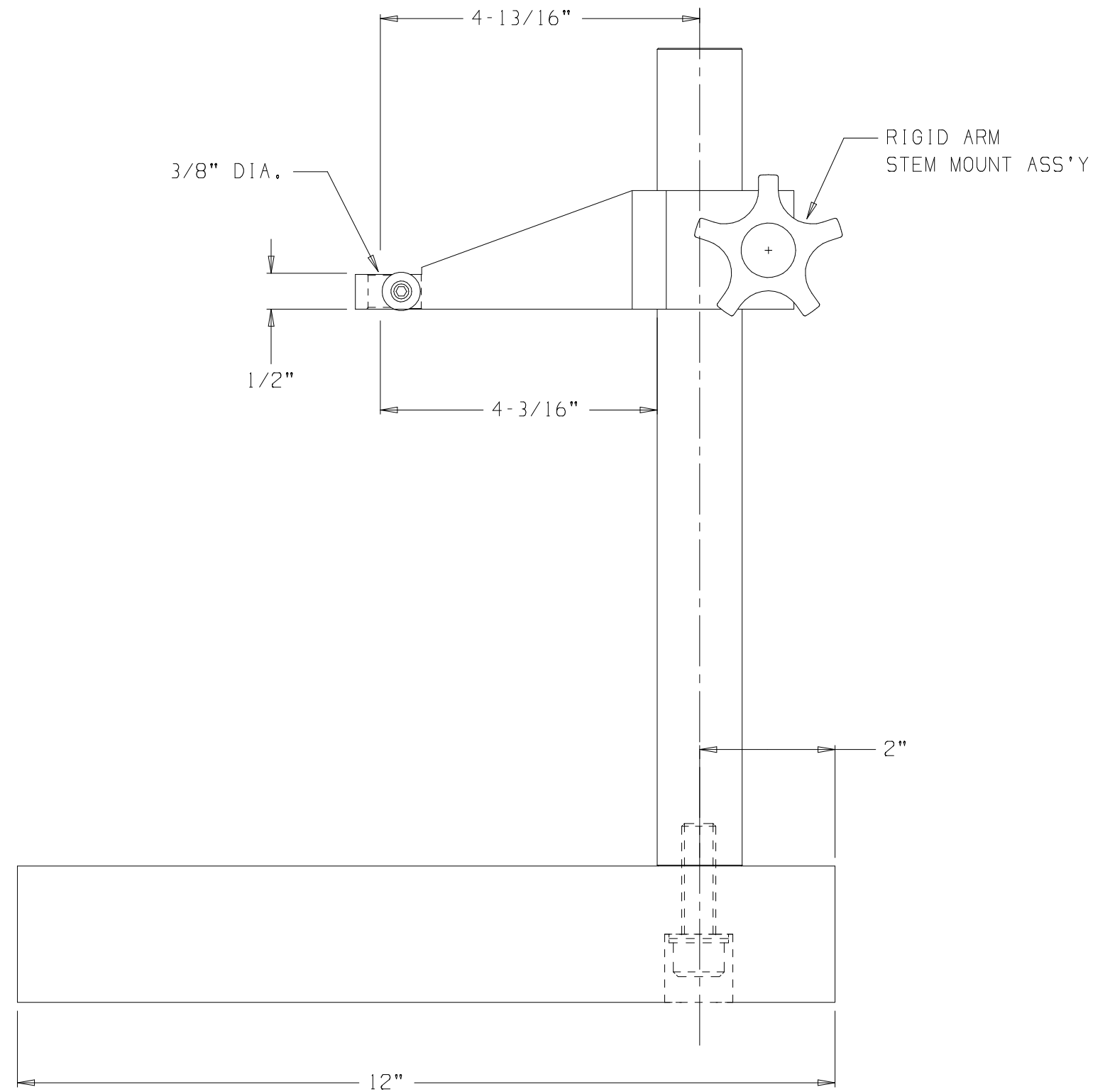
(60812-1RS) GRANITE BASE 8" X 12" X 2" W/RIGID ARM, STEM MOUNT
