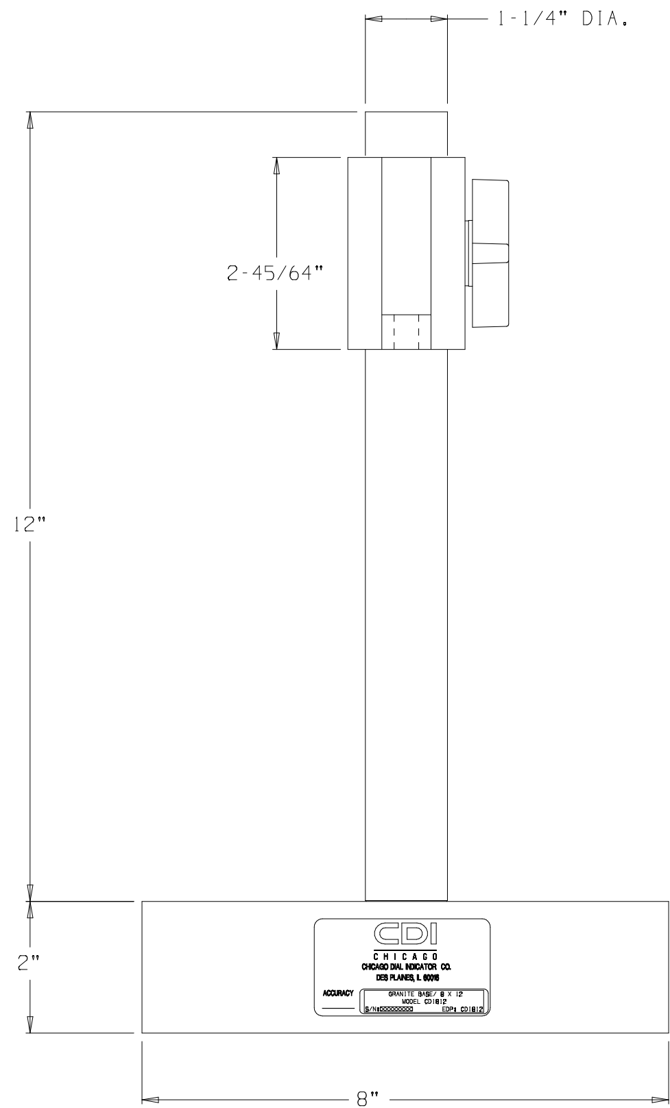
(60812-1RS) GRANITE BASE 8" X 12" X 2" W/RIGID ARM, STEM MOUNT
