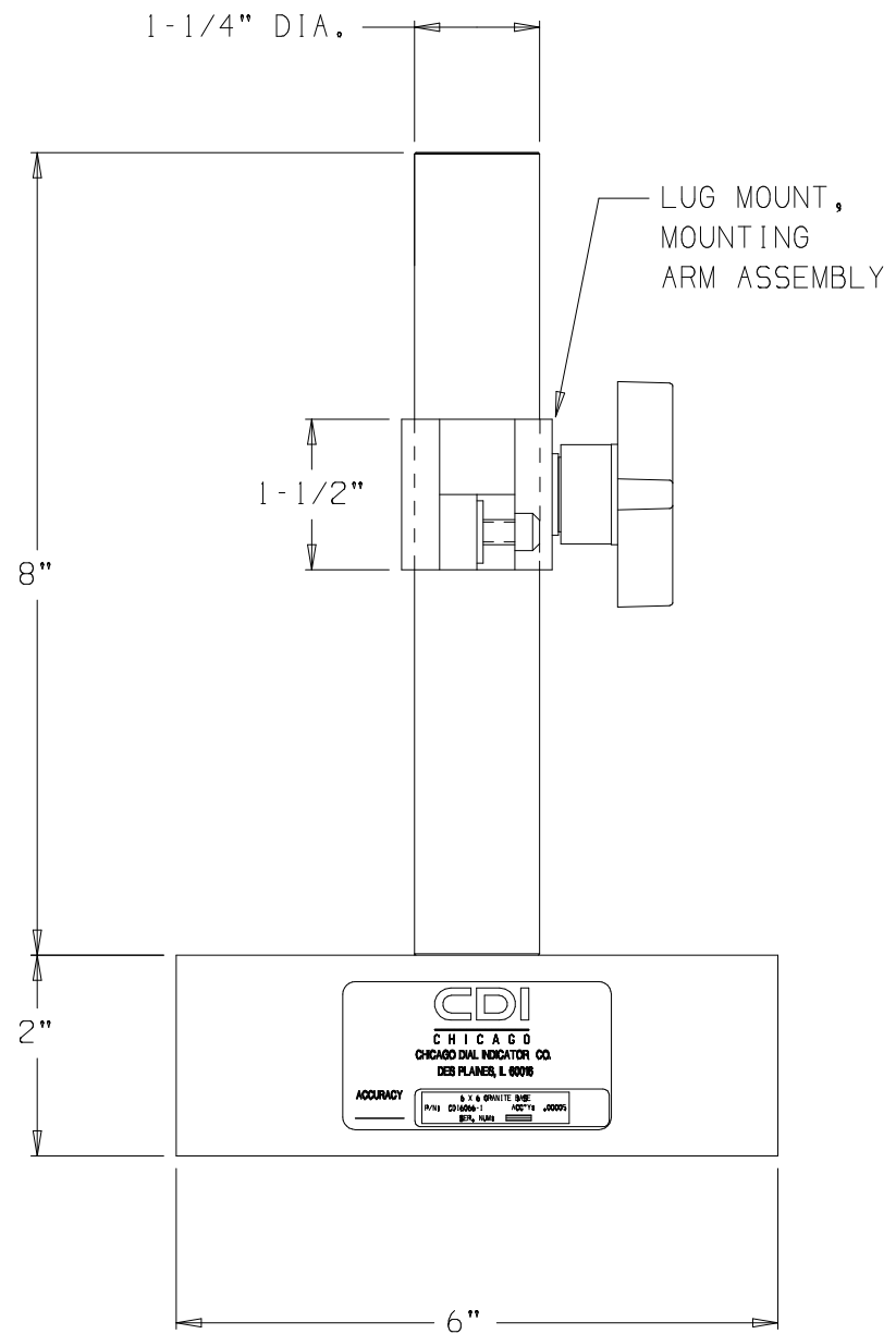
(6066) GRANITE BASE 6" X 6" X 2" W/LUG MOUNT ARM
