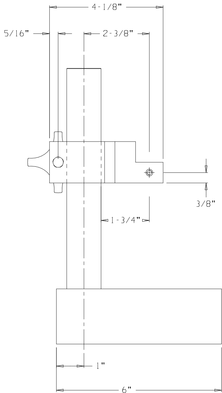
(6066) GRANITE BASE 6" X 6" X 2" W/LUG MOUNT ARM
