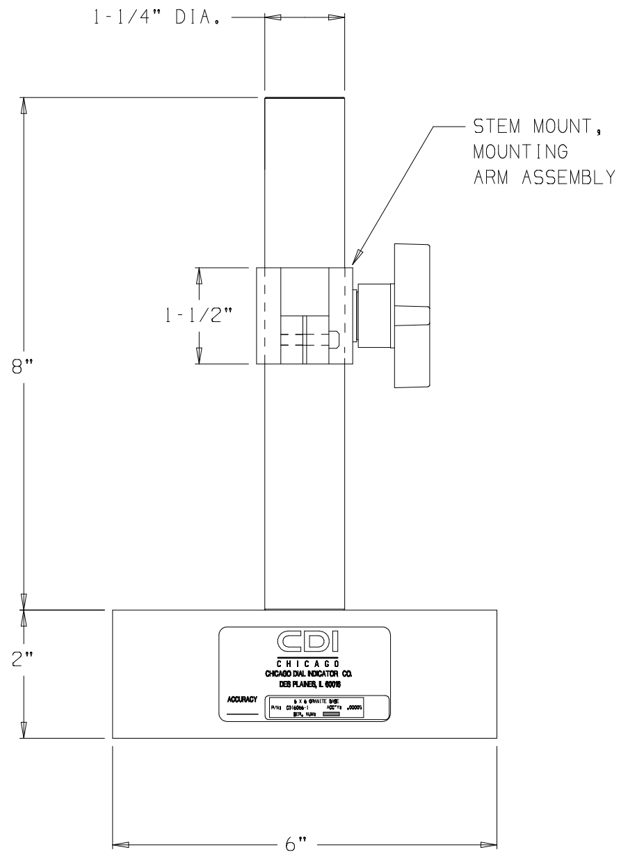
(6066-S) GRANITE BASE 6" X 6" X 2" W/STEM MOUNT ARM
