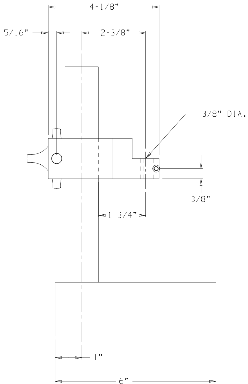
(6066-S) GRANITE BASE 6" X 6" X 2" W/STEM MOUNT ARM
