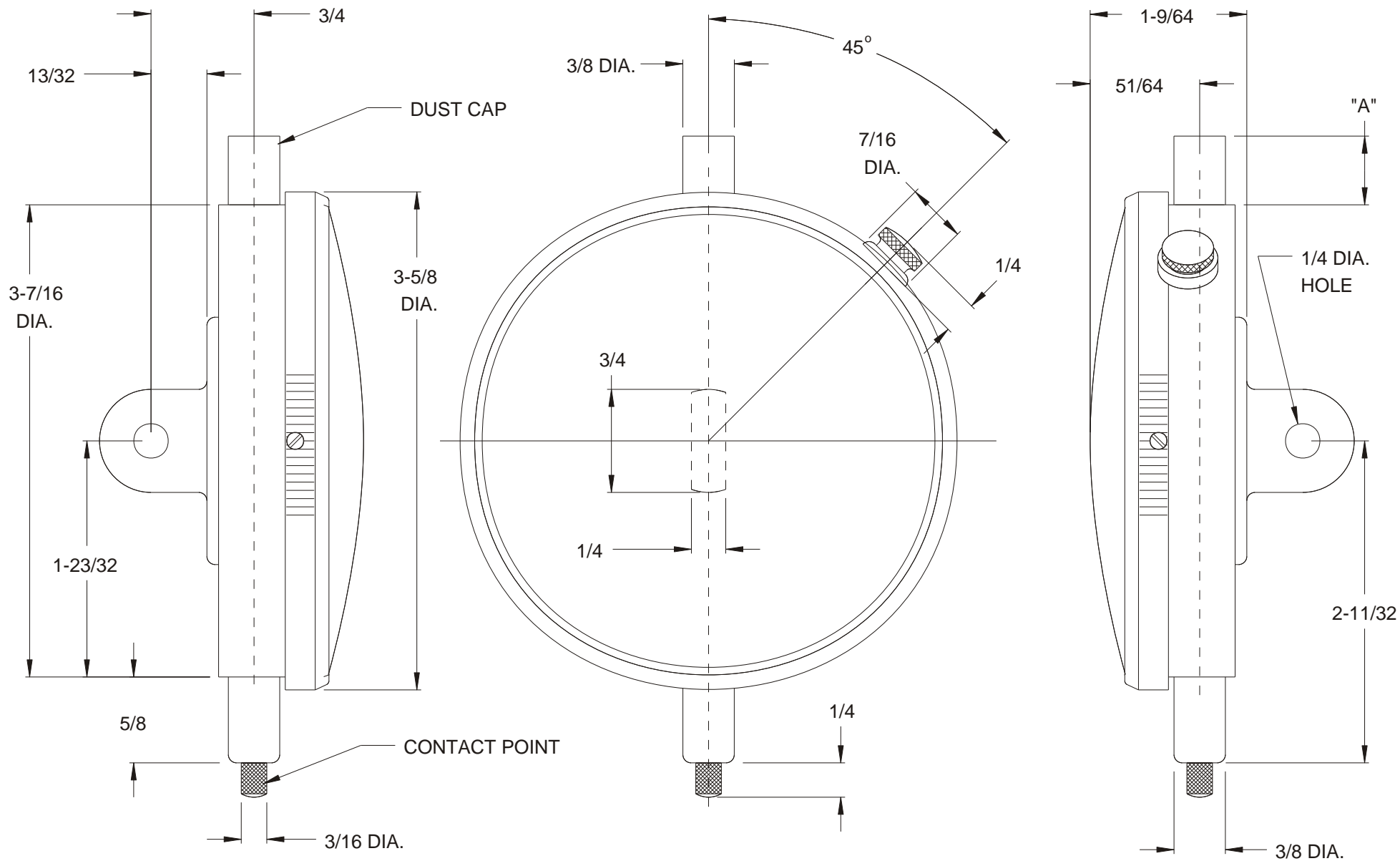
GROUP 4 DIAL INDICATOR UP TO 1" TRAVEL (SHOWN WITH RACK IN UP POSITION)
