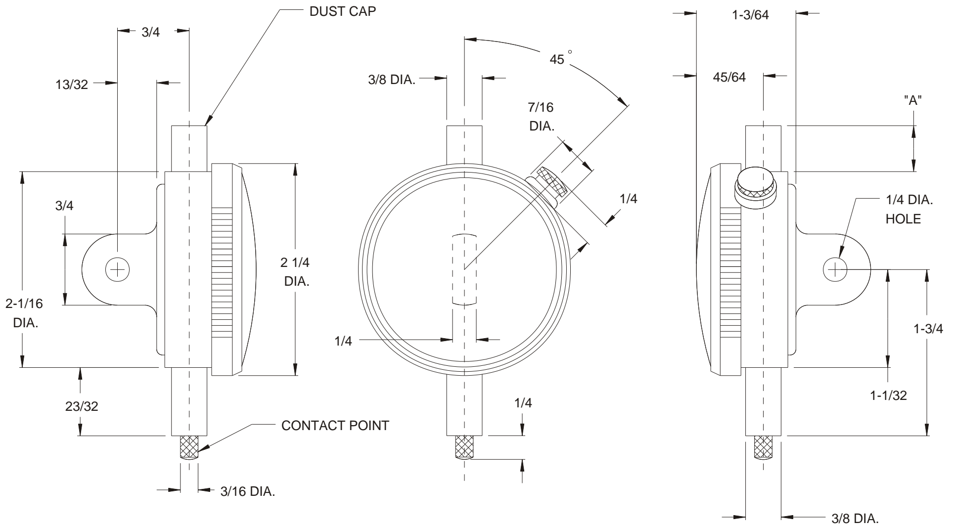
GROUP 2 DIAL INDICATOR UP TO 1" OF TRAVEL (SHOWN WITH RACK IN UP POSITION)
